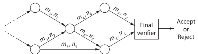
FIGURE 1. A distributed computation in which each party sends a message m_i that is augmented with a short proof \pi_i . The final verifier inspects the computation's outputs in order to decide whether they are “compliant” or not.
