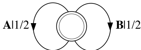
Figure 12 The minimal machine for Figure 11’s internal state process. It has a single state and equal branching probabilities. The topological and statistical complexities are zero and the topological and metric entropies are 1 bit per state symbol — a highly unpredictable, but low complexity process. That this is the correct minimal description of the internal state process follows directly from using machine reconstruction, assuming direct access to the internal state sequences ABABBA .... All state sequences are allowed and those of equal length have the same probability.
