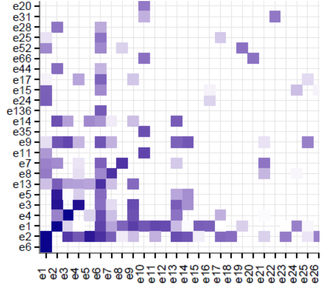
Figure 3 - Heatmap visualizing relationships between files on the attack surface and the frequency of these relationships.
