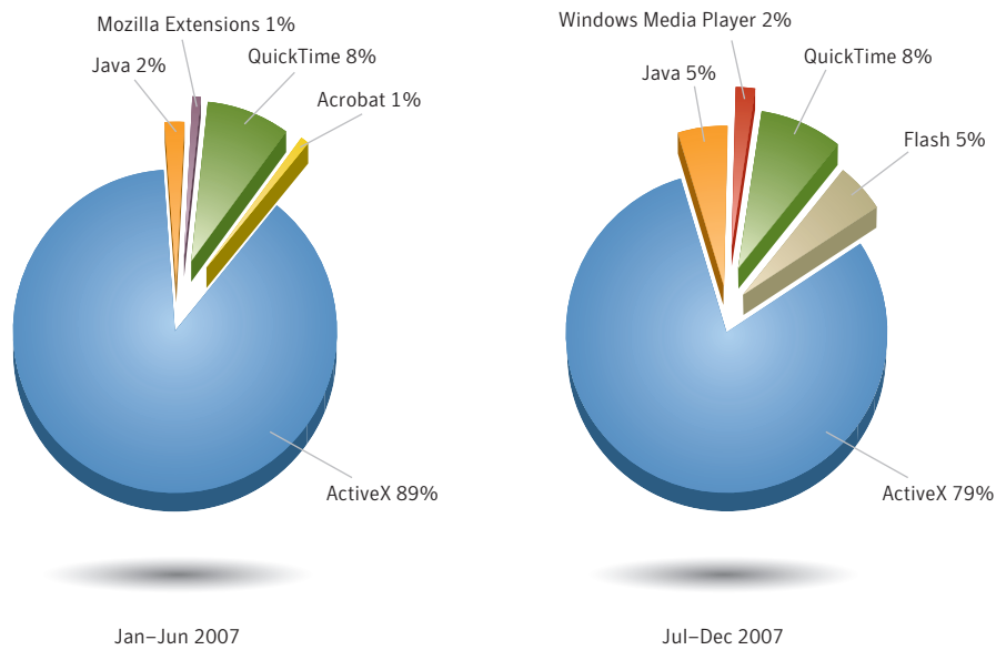
Figure 9. Browser plug-in vulnerabilities Source: Symantec Corporation
