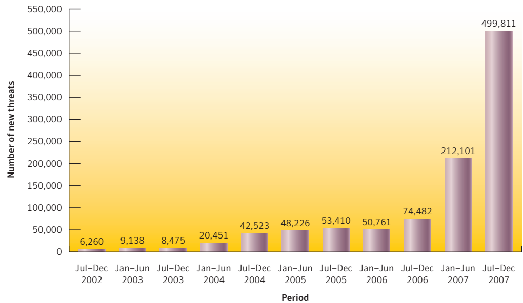
Figure 14. New malicious code threats
